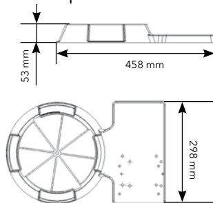
Base plate
