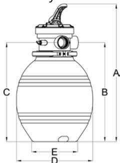
Filterset 300 Body
