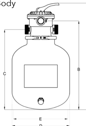
Filterset 400/500/600 Body
